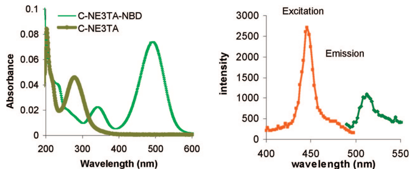
Figure 7. UV and fluorescence spectra of C-NE3TA and C-NE3TA-NBD (10 \mu M, H 2 O).
